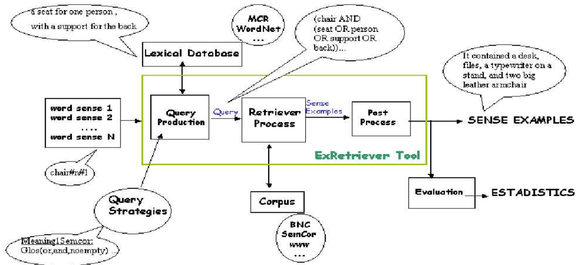
Figure 1: ExRetriever's general schema
