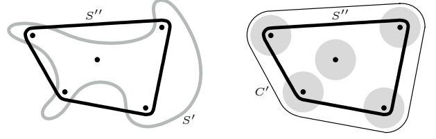
Fig. 3. The sets C', S' and S'' . The black dots indicate the base stations within \text{int}(S') , and the shaded areas around them are neighborhoods of radius l/2 .
