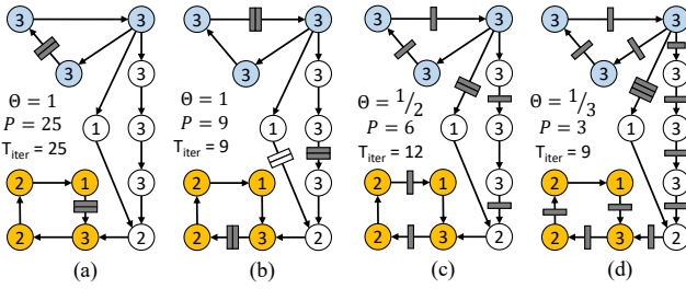
Figure 4: Performance optimization of a choice-free dataflow circuit. Grey buffers are used for breaking combinational paths. The white buffer is transparent and used for throughput optimization.
