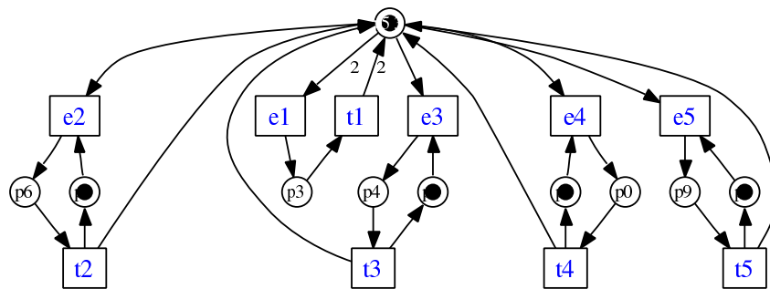
Figure 1.5: Shared resources system: Petri net.
