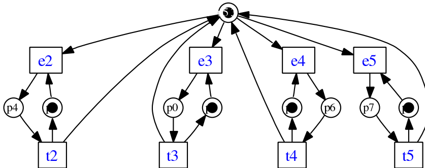
Figure 1.6: Synthesized Petri net on behavior regarding processes P_2 \dots P_5 .
